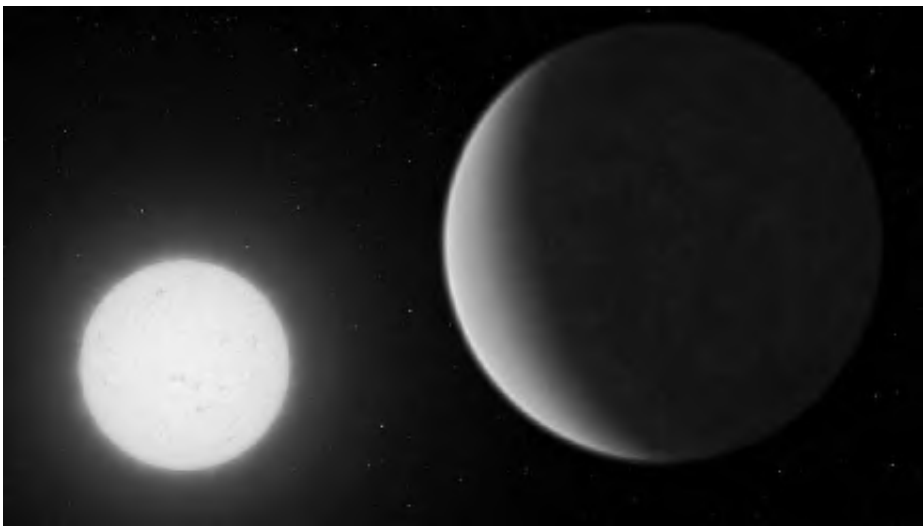
Artist concept of 55 Cancr i e orbiting its nearby host star. Find details from the Spitzer Space Telescope’s close study of its atmosphere at: bit.ly/spitzer55cancr ie and the Hubble Space Telescope’s observations at bit.ly/hubble55cancr ie Credit: NASA/JPL-Caltech
